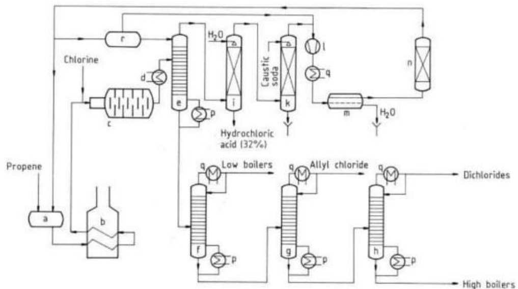
Gambar 1.2 Flowsheet dasar chlorinasi propylene
