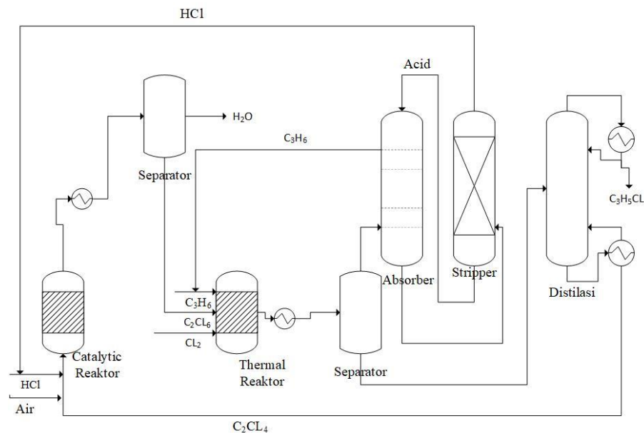
Gambar 1.3 Flowsheet dasar oxychlorination propylene
