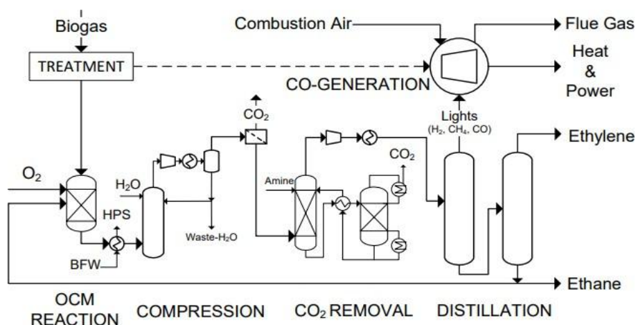
Gambar 1.7 Flow Diagram Proses Oxidative Coupling of Methane (OCM)
